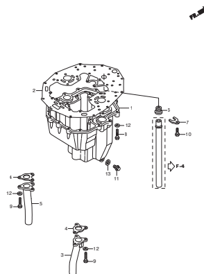
E-6 OIL PAN
