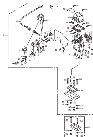
FOP-3 REMOTE CONTROL (TOP MOUNT SINGLE TYPE) (RIGHT)
