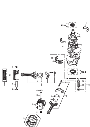
E-7 CRANKSHAFT/PISTON
