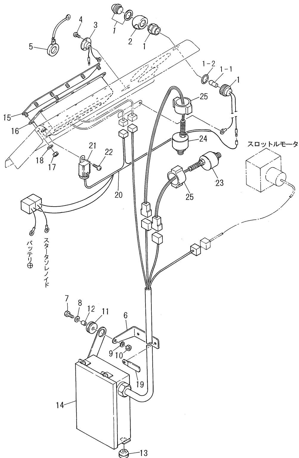
電装 Fig. 8 ELECTRICAL EQUIPMENT
